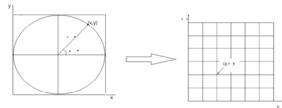
Figure1. Transformation from Cartesian coordinate to Log-polar coordinate.
