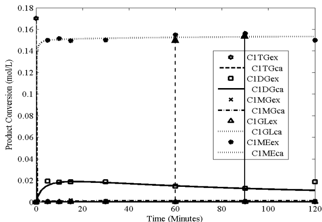
Fig4.eps, Conversion versus time. Temperature = 65°C, stirring rate = 700 rpm; molar ratio = 6:1 and catalyst loading = 1%
