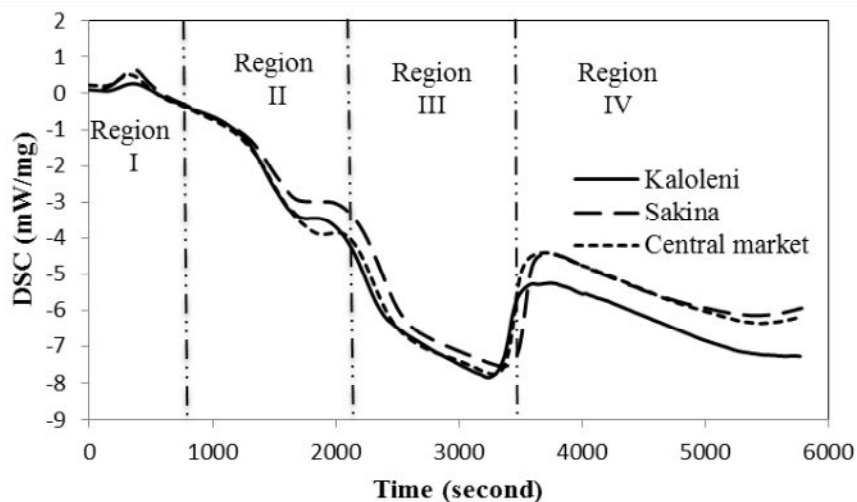
Figure 4: DSC of Arusha Municipal solid waste sites.
