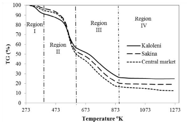
Figure 1: TG of Municipal solid waste
