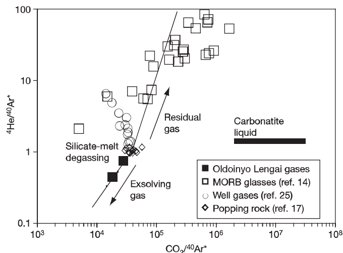
Figure 3 | ^4\text{He}/^{40}\text{Ar}^* and \text{CO}_2/^{40}\text{Ar}^* ratios of Oldoinyo Lengai gases. New Mexico well-gas data 25 and compositions of 2IID43 popping rock are considered representative of the volatile compositions of primary mantle melts 17 . The volatile composition of a carbonatite liquid in equilibrium with such a primary melt is calculated using a mass-balance approach (Supplementary Information). Rayleigh-type degassing will fractionate the exsolved volatiles from the initial volatile compositions (defined by popping rock for silicate magmas and the calculated carbonatite pole for carbonatitic magmas), with the exsolving gases moving towards lower ^4\text{He}/^{40}\text{Ar}^* and \text{CO}_2/^{40}\text{Ar}^* values owing to higher solubility of He (ref. 21) and \text{CO}_2 (ref. 33) relative to Ar (ref. 21) in the melt. MORB glasses 14 have compositions that represent the residual mantle gas after degassing. The models show that volatiles sampled at Oldoinyo Lengai could not have been exsolved from a carbonatite magma and instead coincide with the compositions expected from a degassing silicate magma.
