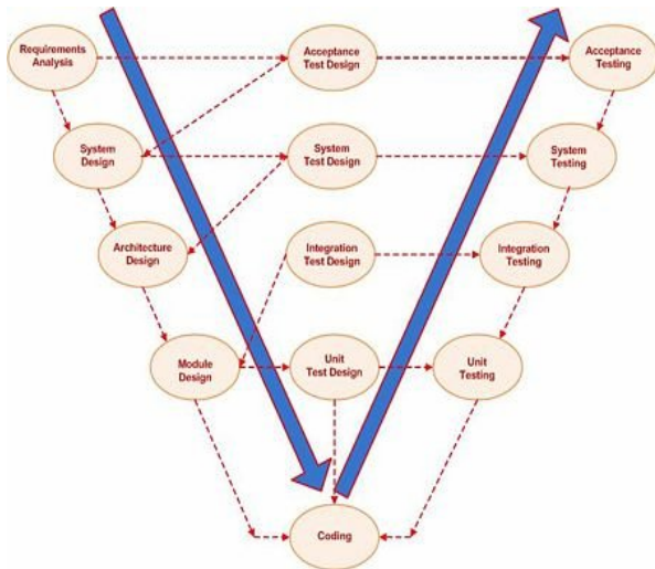
Fig. 2 V-Model Software Development Process (Software life cycle)
