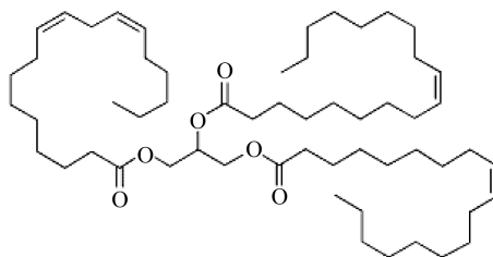
Figure 4. 1,2-OLEIN-3-LINOLEIN chemical structure.
