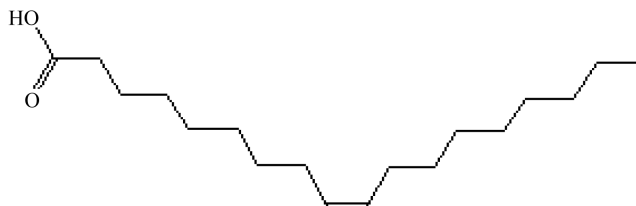
Figure 5. Oleic acid chemical structure.
