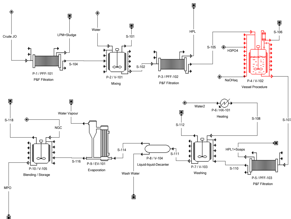
Figure 1. Process flow diagram (PFD) of MPO production obtained from superpro designer.
