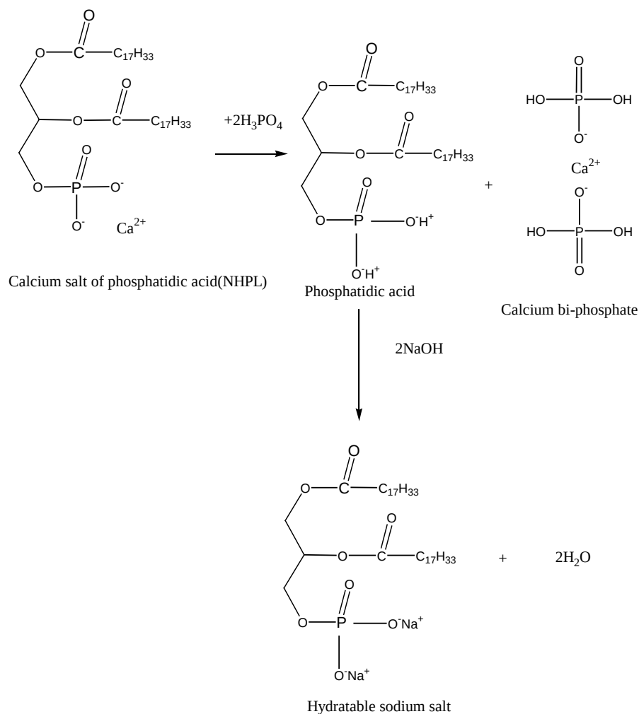
Figure 2. Acid Degumming and partial neutralisation [36].
