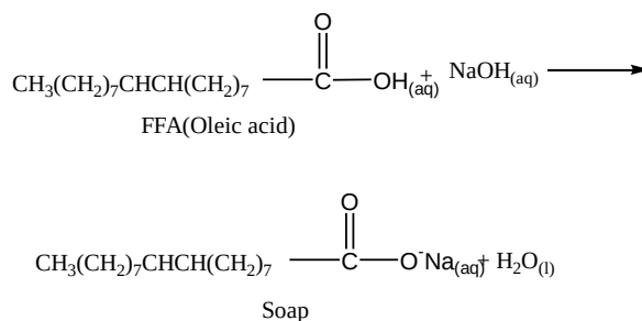
Figure 3. Saponification or neutralisation reaction.
