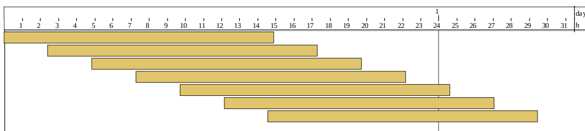
Figure 7. Gantt chart.
