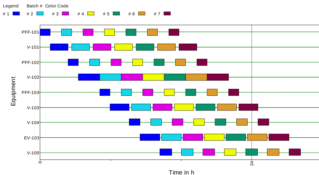
Figure 6. Equipment utilisation chart.
