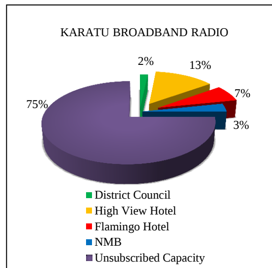
Figure 5. Bandwidth Capacity Utilization of the Longido Radio Link
