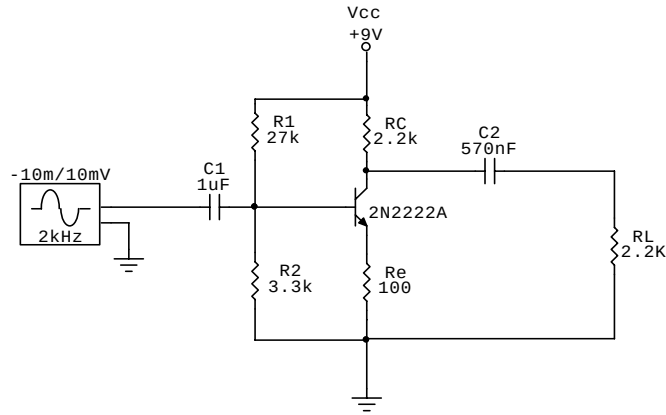
Figure 10: Single Stage Common Emitter Amplifier used at UDSM.
