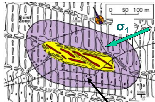
Figure 3. Mine layout showing major far field stress orientation relative to orebody and orientation of pillars (after Martin and Maybee, 2001).
