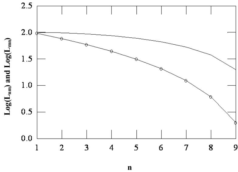
Fig. 9: Variation of L_{nm} and L_{mn} with n at N=16 and increasing P_2...P_{N-1} (—) and Q_2...Q_{N-1} (—o—).
