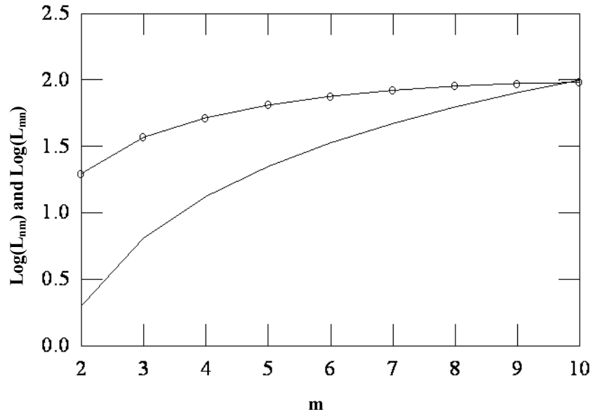
Fig. 10: Variation of L_{nm} and L_{mn} with m at N=16 and increasing P_2...P_{N-1} (—) and Q_2...Q_{N-1} (—o—).
