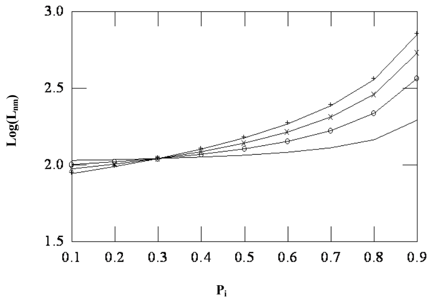
Fig. 7: Variation of L_{mn} with P_{nn} (—), P_{22}...P_{nn} (x), P_{nn}...P_{mm} (○) and P_{22}...P_{N-1,N-1} (+) at n = 6 , m = 11 and N = 16 .
