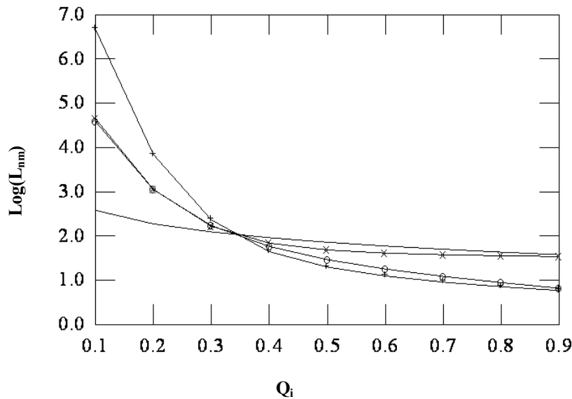
Fig. 8: Variation of L_{nm} with Q_n (—), Q_2 \dots Q_n (—x—), Q_n \dots Q_m (—○—) and Q_2 \dots Q_{N-1} (—□—) at n = 6 , m = 11 and N = 16 .
