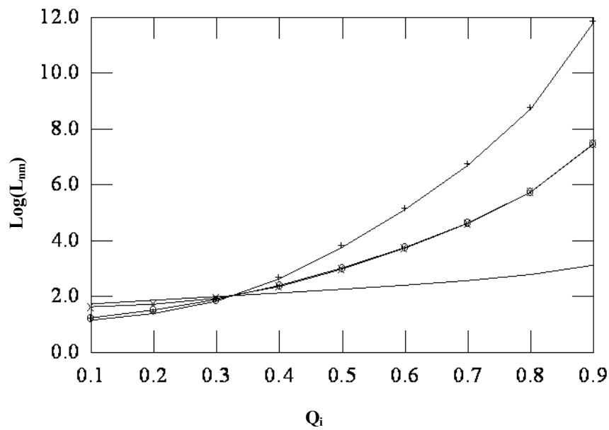
Fig. 5: Variation of L_{nm} with Q_n (—), Q_2...Q_n (—x—), Q_n...Q_m (—o—) and Q_2...Q_{N-I} (—+—) at n = 6 , m = 11 and N = 16 .
