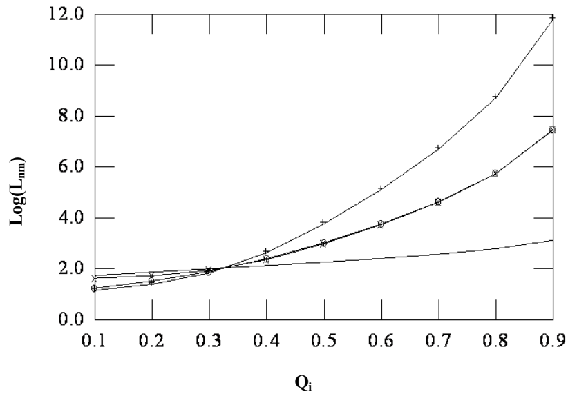
Fig. 6: Variation of L_{mn} with P_n (—), P_2...P_n (x), P_n...P_m (○) and P_2...P_{N-1} (+) at n = 6 , m = 11 and N = 16
