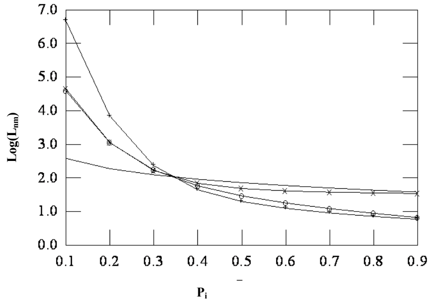
Fig. 3: Variation of L_{nm} with P_n (—), P_2...P_n (—x—), P_n...P_m (—o—), and P_2...P_{N-1} (—+—) at n = 6 , m = 11 and N = 16 .
