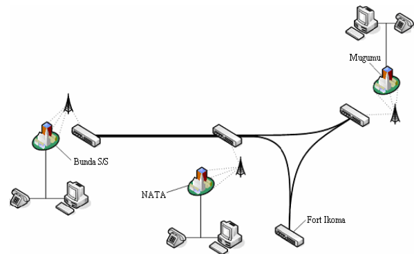
Fig. 5 Logical network diagram of Bunda to Mugumu connection [18]
