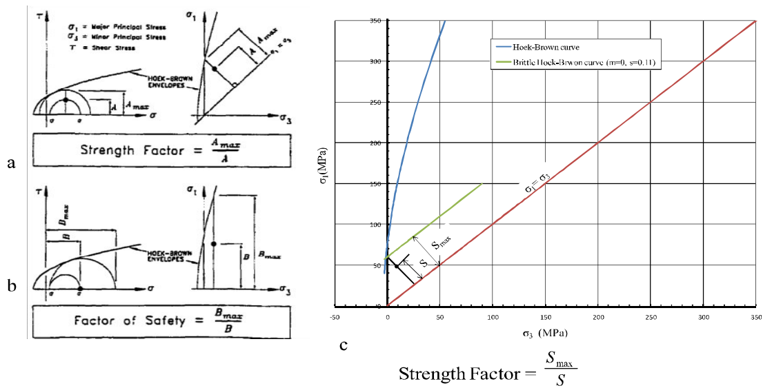
Figure 3: (a) Strength factor (b) factor of Safety (McCreath and Diederichs, 1994) (c) definition of strength factor using Brittle Hoek-Brown parameters to be used in this paper
