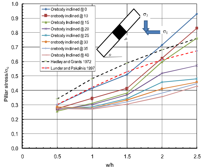
Figure 6: Comparison of pillar stability charts for different orebody inclinations ( k=1.5 , R=75\% , FS=1 )
