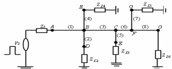
Fig. 2 Power line network with three distributed branches
