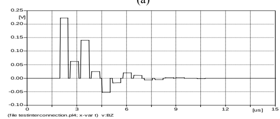
Fig. 3 Simulation Results (a) Model Result (b) ATP-EMTP Results
