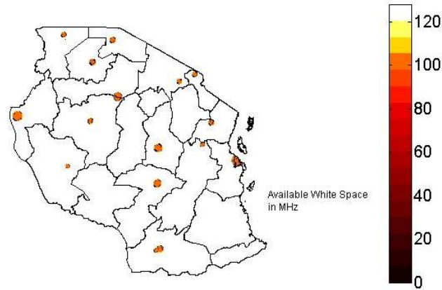
Fig. 2. TV White Space availability using Pollution viewpoint \gamma = 15\text{dB}
