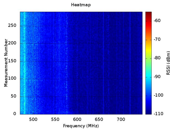
Fig. 6. Spectrum utilization graph for data collected at Ibihwa Dispensary (-6.005, 35.432), Bahi District Council using handheld spectrum analyzer.
