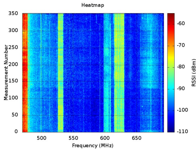
Fig. 4. Spectrum utilization graph for data collected at Nyerere Square (-6.178, 35.748), Dodoma Municipal Council using handheld spectrum analyzer.
