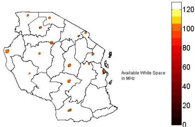
Fig. 3. TV White Space availability using Protection viewpoint \Delta = 1\text{dB}
