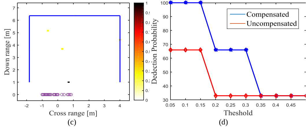
Figure 7: Reconstructed image (a) Original scene (b) Uncompensated (c) Path loss compensated (d) Detection probability for compensated and uncompensated images.
