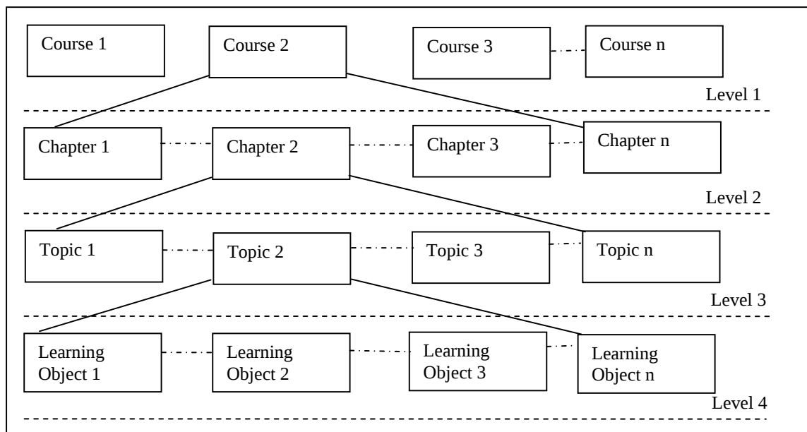
Fig. 3 Courseware Tree
