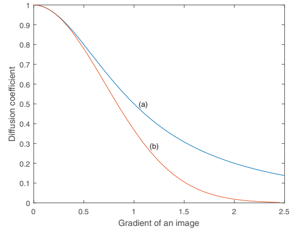
Figure 1: Perona-Malik diffusion coefficients with shape-defining constant, K = 1 : (a) \phi_1(s) = \frac{1}{1 + \left(\frac{s}{K}\right)^2} , and (b) \phi_2(s) = \exp(-(s/K)^2) .
