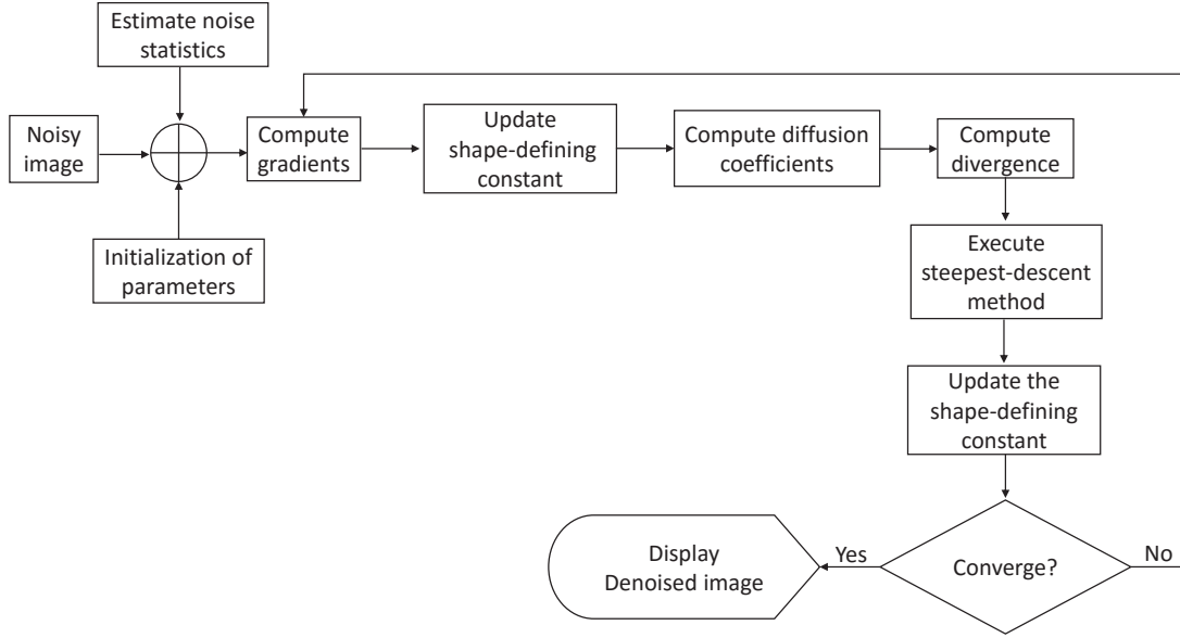
Figure 3: Automated Perona-Malik denoising method.
