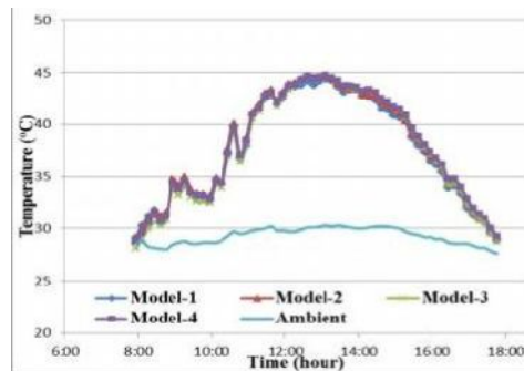
Figure 15: Temperature profile of collector with same glass thickness
