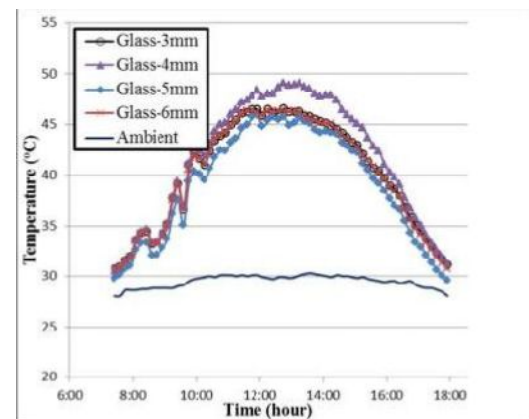
Figure 16: Temperature profiles of collector with different glass thickness
