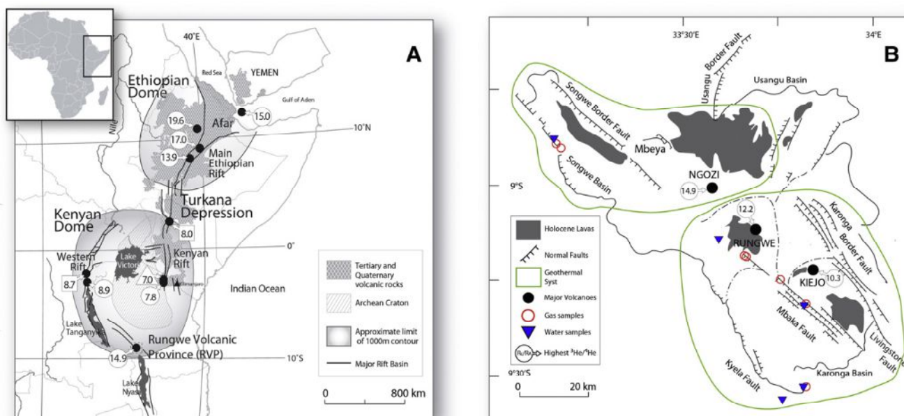
Fig. 1. A – Left: the location of the EARS (after Hilton et al., 2011 ). The highest reported ^3\text{He}/^4\text{He} ratios are plotted for various segments of the EARS, using circles (lavas), squares (hydrothermal fluids) and triangles (xenoliths). In the Western Rift of the Kenyan Dome region, ^3\text{He}/^4\text{He} ratios do not exceed canonical MORB values ( 8 \pm 1 R_A ) with the exception of high ^3\text{He}/^4\text{He} phenocryst values from RVP ( Hilton et al., 2011 ). In addition, high He-isotopes ( ^3\text{He}/^4\text{He} > \text{MORB} ) are observed in the Ethiopia Dome, nearly 2000 km north of RVP ( Scarsi and Craig, 1996 ) and extend throughout the Afar region to the Gulf of Aden, Red Sea and Yemen ( Marty et al., 1996 ). B – Right: enlarged map of RVP with sample locations, fault systems, lava outcrops, major volcanoes and the main hydrothermal systems (e.g., Ngozi-Songwe in the north, Kiejo-Mbaka in the south). Open red circles denote gas samples and blue inverted triangles represent fluids samples. For reference, the highest measured ^3\text{He}/^4\text{He} values ( Hilton et al., 2011 ) at RVP are shown inside circles for each of the three main volcanic centers.
