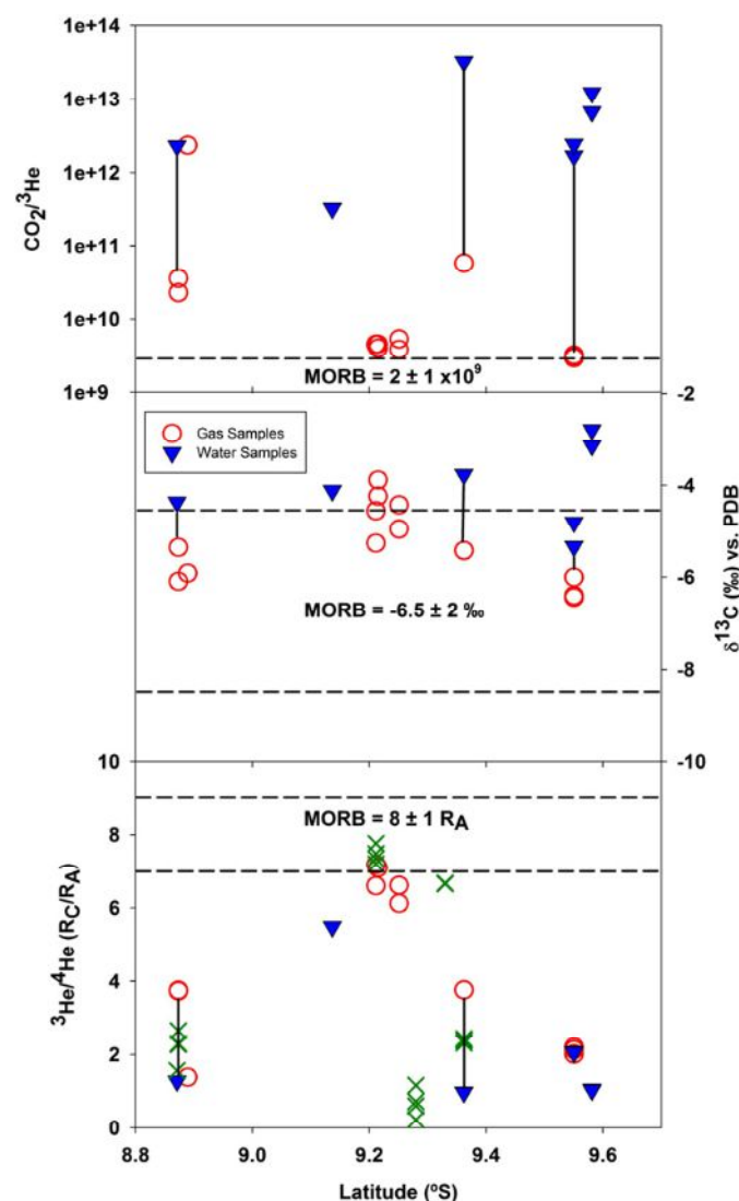
Fig. 3. Helium and carbon isotope ( ^3\text{He}/^4\text{He} – corrected for air and given in R_C/R_A notation; \delta^{13}\text{C} ) and relative abundances ( \text{CO}_2/^3\text{He} ) plotted versus latitude for all 11 RVP localities sampled. Open red circles represent gas-phase samples and solid blue triangles represent fluid-phase samples. In addition, hydrothermal fluid He-isotopes (from Pik et al., 2006) are shown (green X's). Vertical tie-lines connect gas and fluid phase samples from the same locality. Horizontal dashed lines delineate typical MORB ranges for carbon and helium isotopes.
