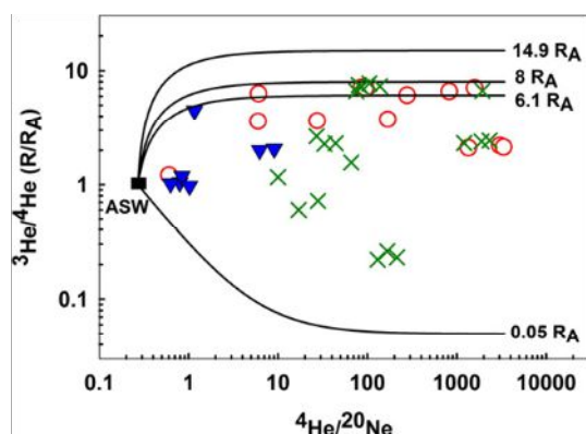
Fig. 2. He-isotopes versus ^4\text{He}/^{20}\text{Ne} data for hydrothermal fluids (blue inverted triangles) and gases (red open circles) from RVP. Data are shown with previously reported hydrothermal fluid data (green X's) from Pik et al. (2006). Calculated binary mixing lines between air saturated water (ASW), crustal and mantle endmember compositions are shown. Endmembers are: ASW ^3\text{He}/^4\text{He} = 1 R_A , ^4\text{He}/^{20}\text{Ne} = 0.250\text{--}0.285 ; (Ozima and Podosek, 1983), High ^3\text{He}/^4\text{He} = 14.9 R_A , (Hilton et al., 2011), MORB ^3\text{He}/^4\text{He} = 8 R_A , (Graham, 2002), SCLM ^3\text{He}/^4\text{He} = 6.1 R_A , (Gautheron and Moreira, 2002) Crustal ^3\text{He}/^4\text{He} = 0.05 R_A (Morrison and Pine, 1955); in the latter 4 cases a ^4\text{He}/^{20}\text{Ne} ratio ~3500 is assumed.
